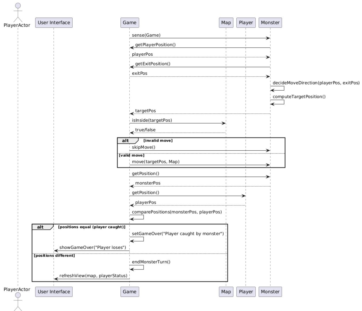
Figure 3.3 Sequence Diagram – Monster Turn
