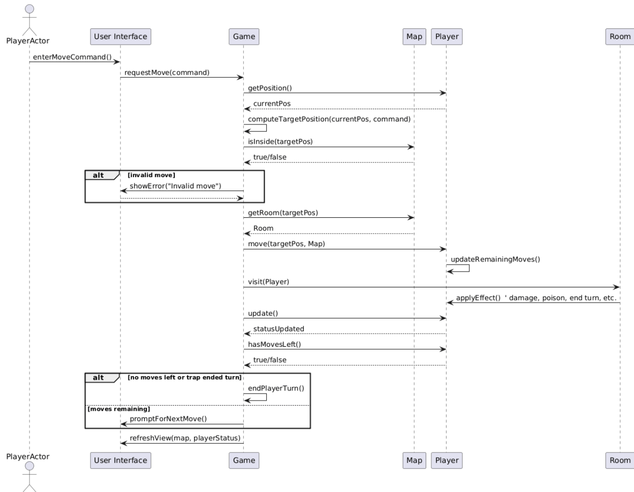
Figure 3.2 Sequence Diagram – Player Turn
