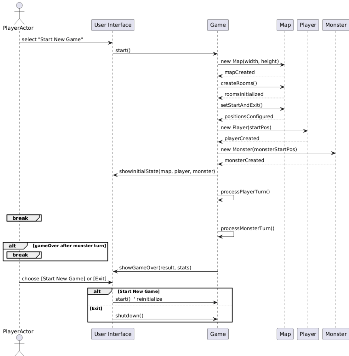
Figure 3.4 Sequence Diagram – Game Initialization
